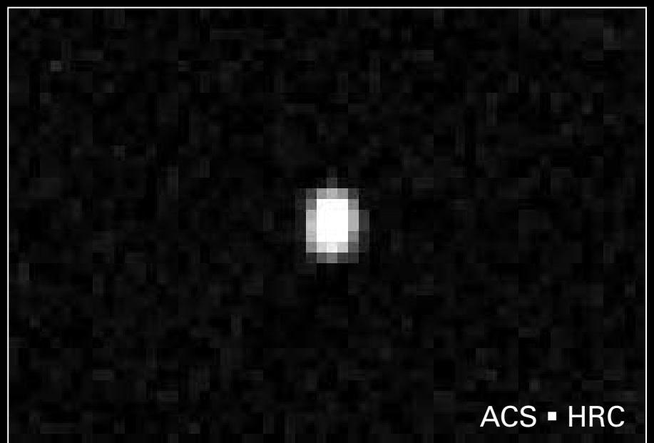
Kuiper Belt Object "Quaoar" Hubble Space Telescope ■ Advanced Camera for Surveys
