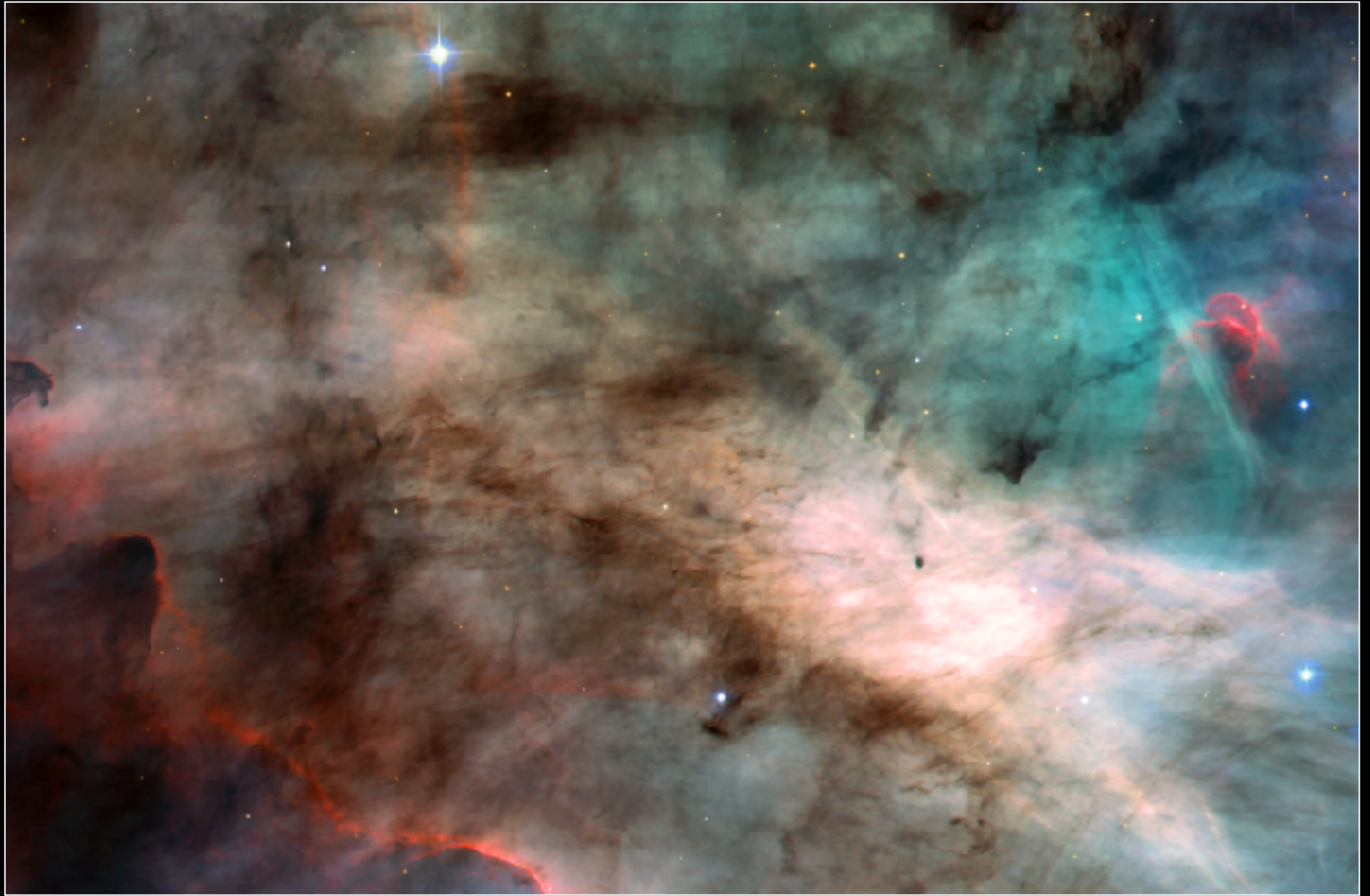
The Omega Nebula • M17 Hubble Space Telescope • Advanced Camera for Surveys
