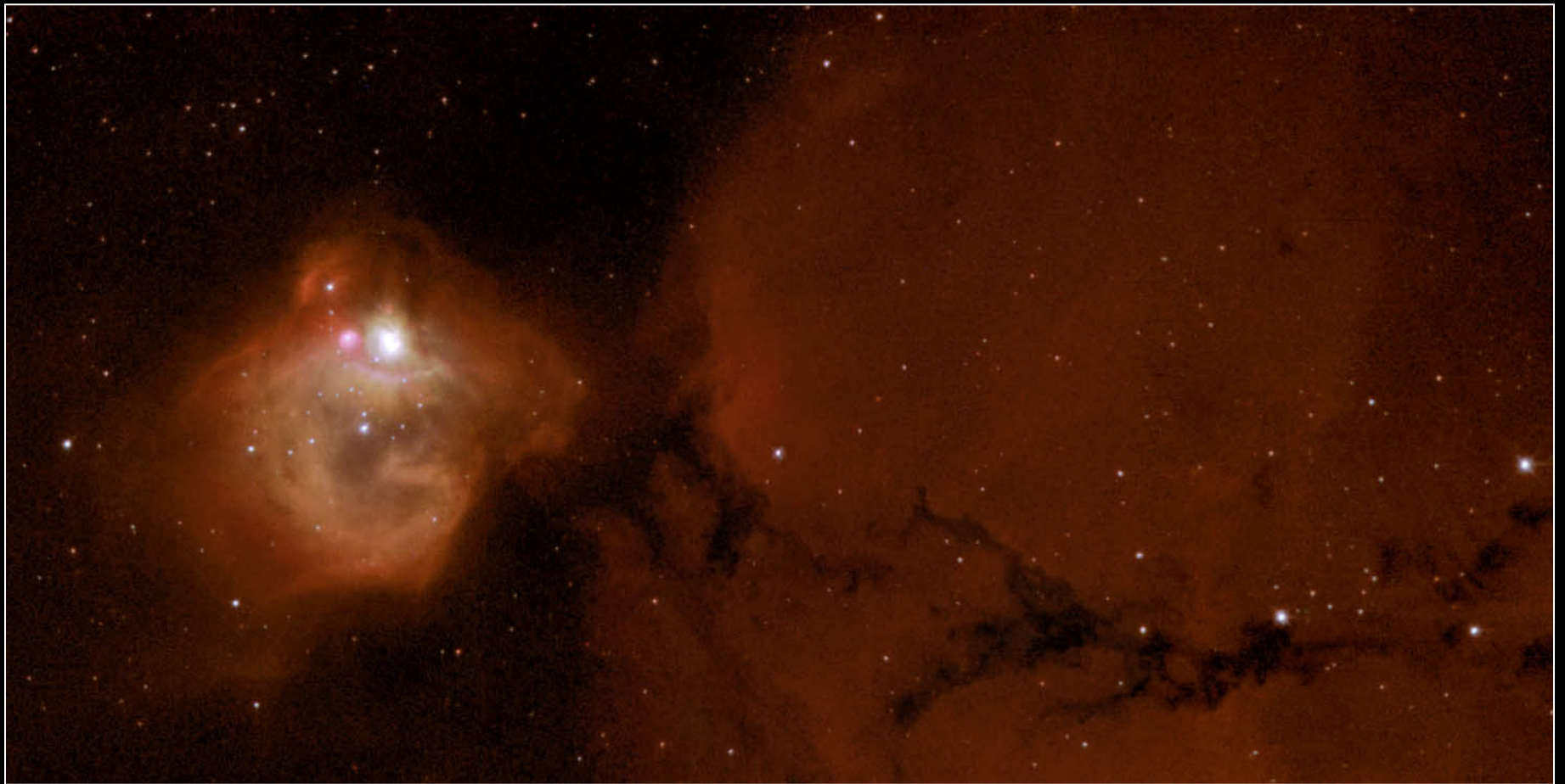
Nebula N83B (NGC 1748) in the Large Magellanic Cloud Hubble Space Telescope • WFPC2
