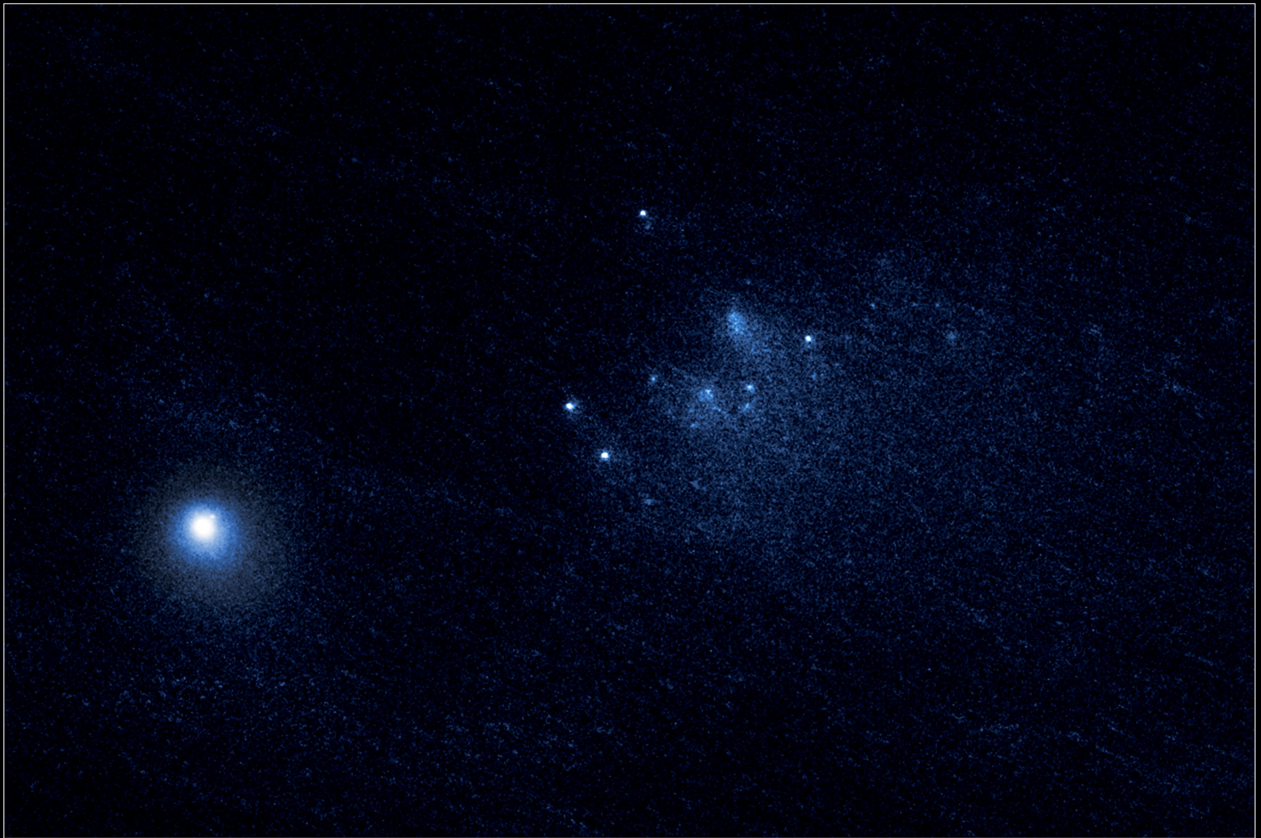
Comet 332P/Ikeya-Murakami Hubble Space Telescope ■ WFC3/UVIS
