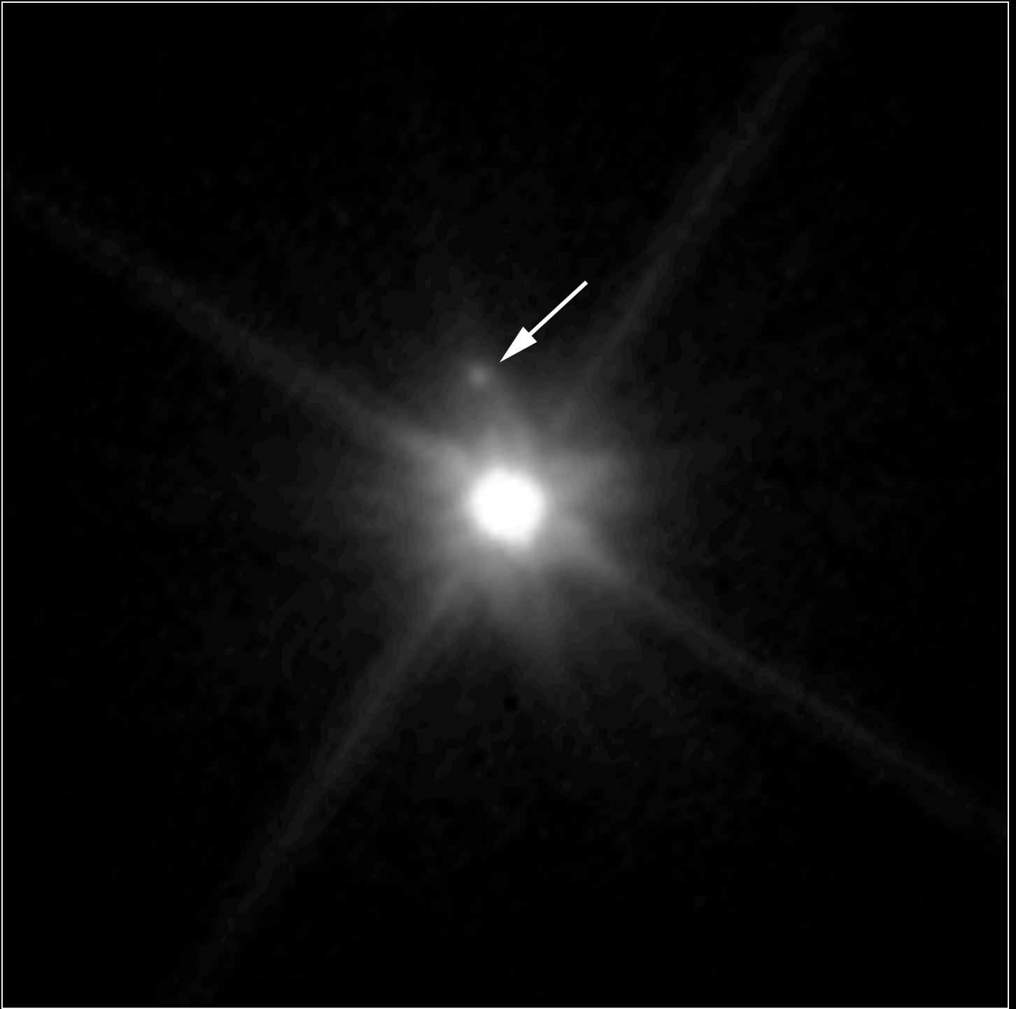
Dwarf Planet Makemake and Moon Hubble Space Telescope ■ WFC3/UVIS
