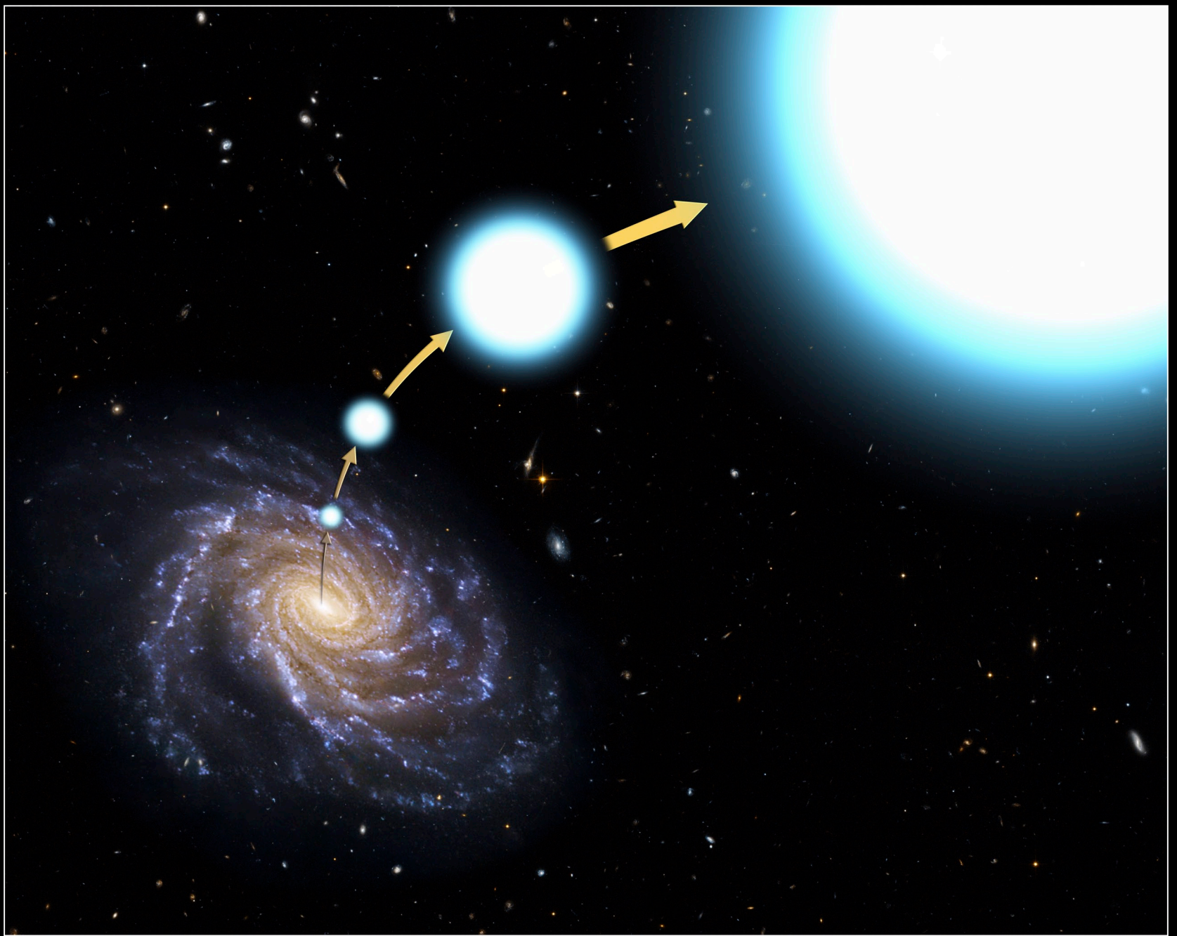
Artist's View of Hypervelocity Star HE 0437-5439
