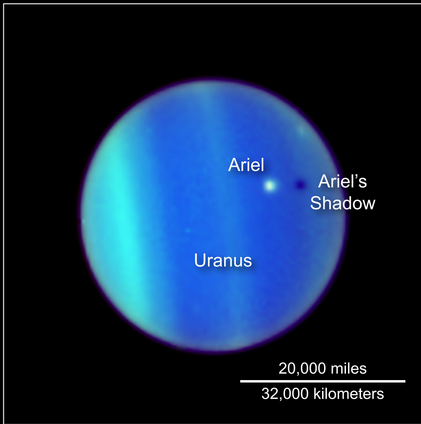
Uranus and Ariel Hubble Space Telescope ■ ACS/WFC
