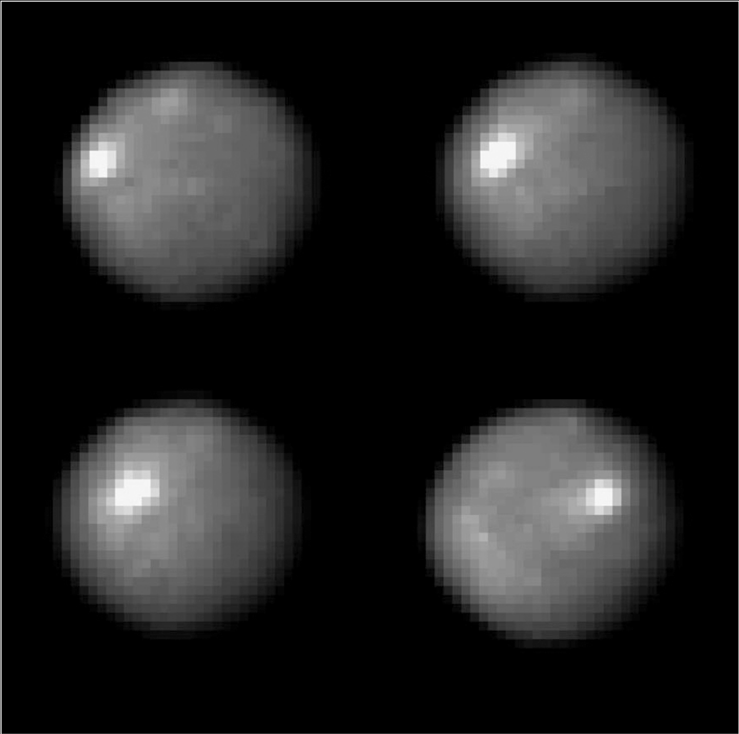
Asteroid 1 Ceres Hubble Space Telescope • ACS/HRC
