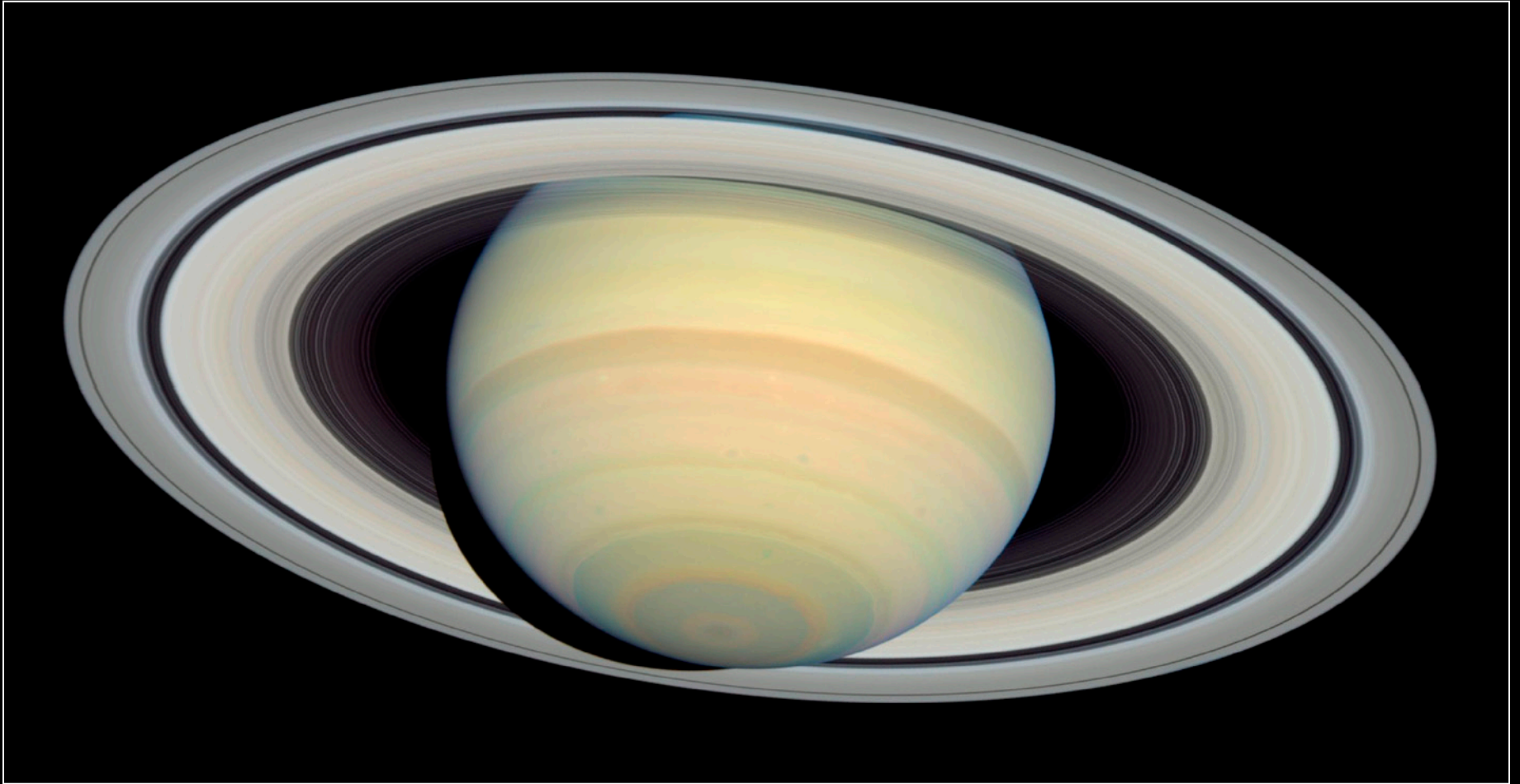
Saturn • March 22, 2004 Hubble Space Telescope • ACS
