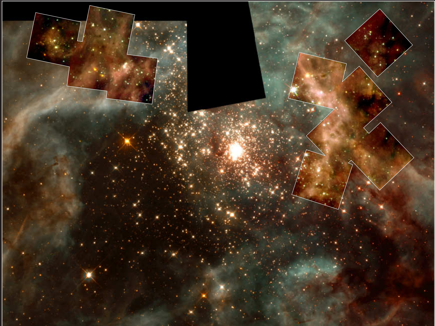
30 Doradus Nebula • Large Magellanic Cloud Hubble Space Telescope • WFPC2 • NICMOS
